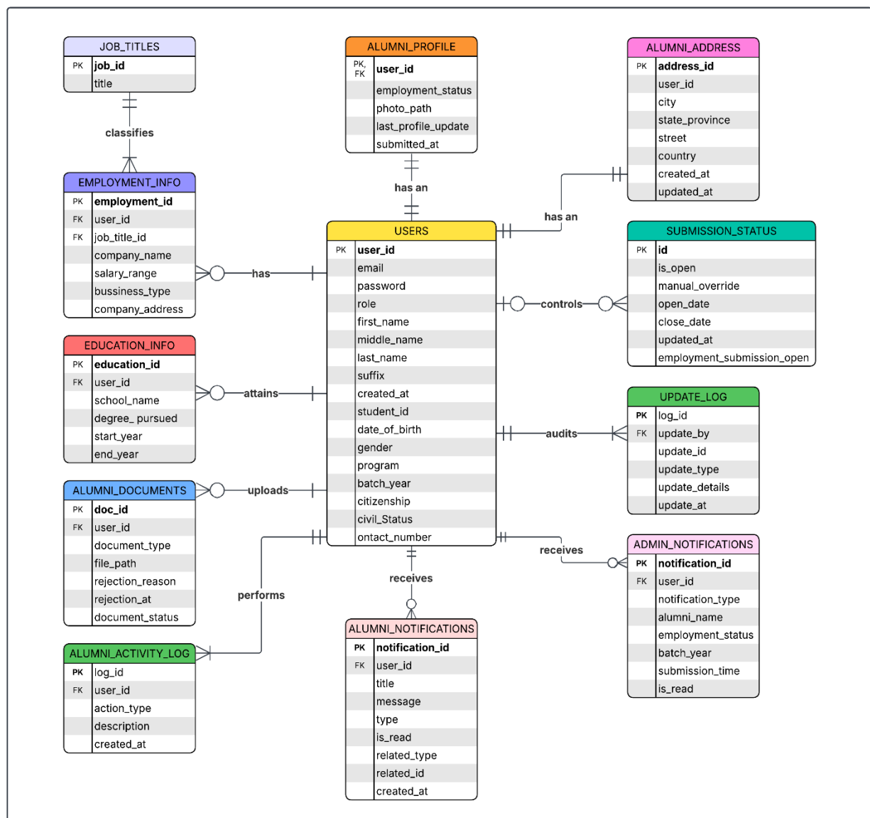
Figure 3.2. Entity-Relationship Diagram
